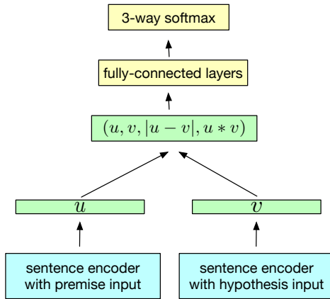
Figure 1: Generic NLI training scheme.
